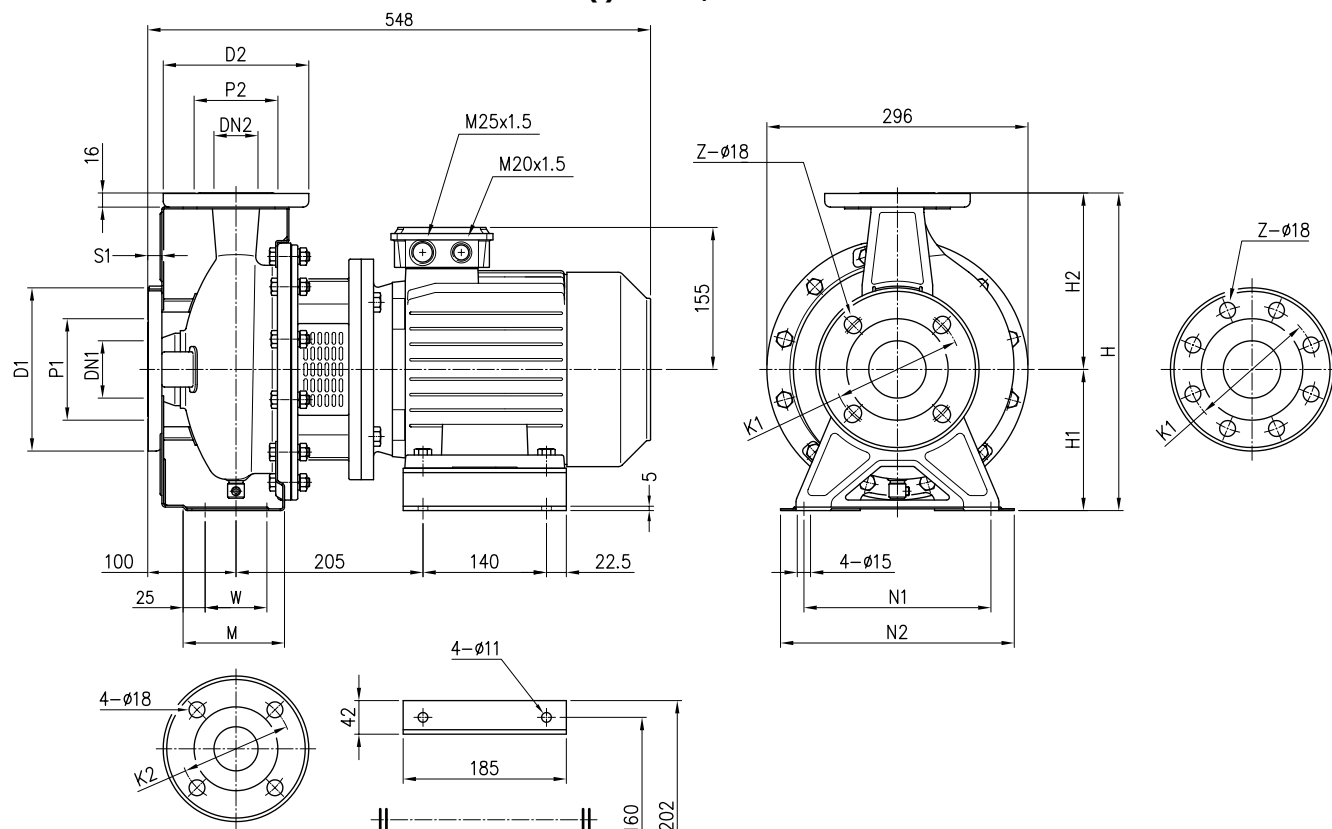
PUMP 3(.)S4 50, 65-160/200
