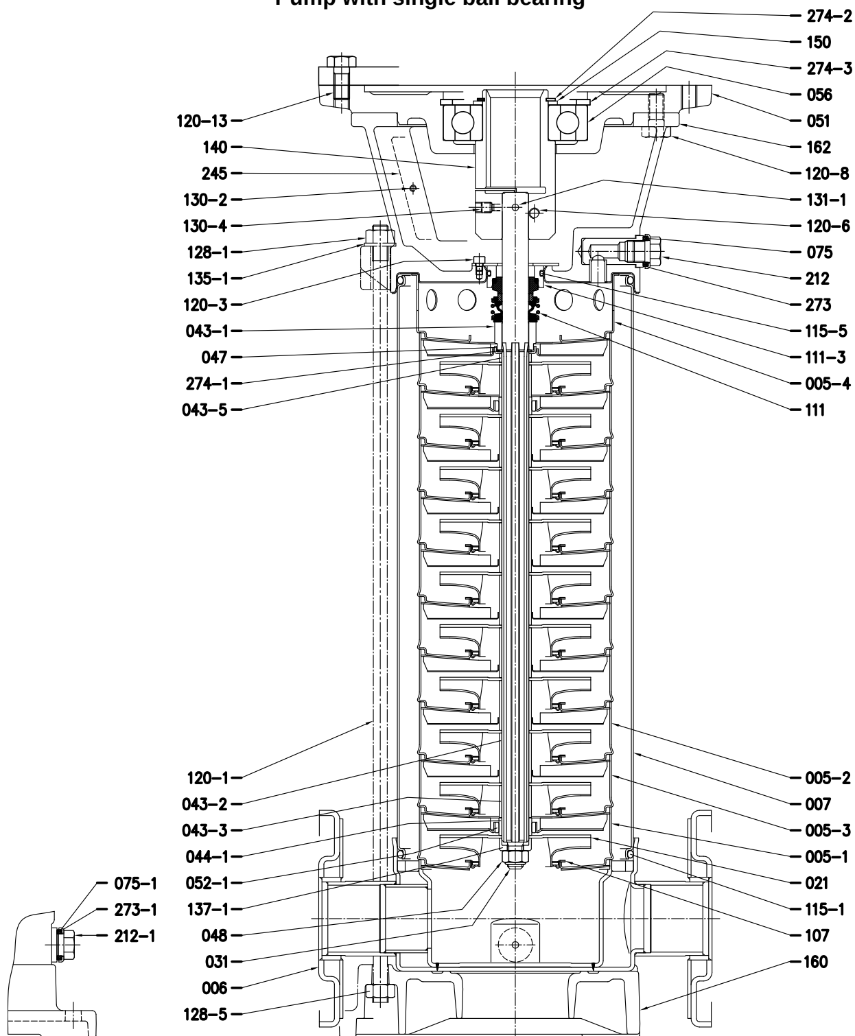
EVM(.) 18 Pump with single ball bearing
