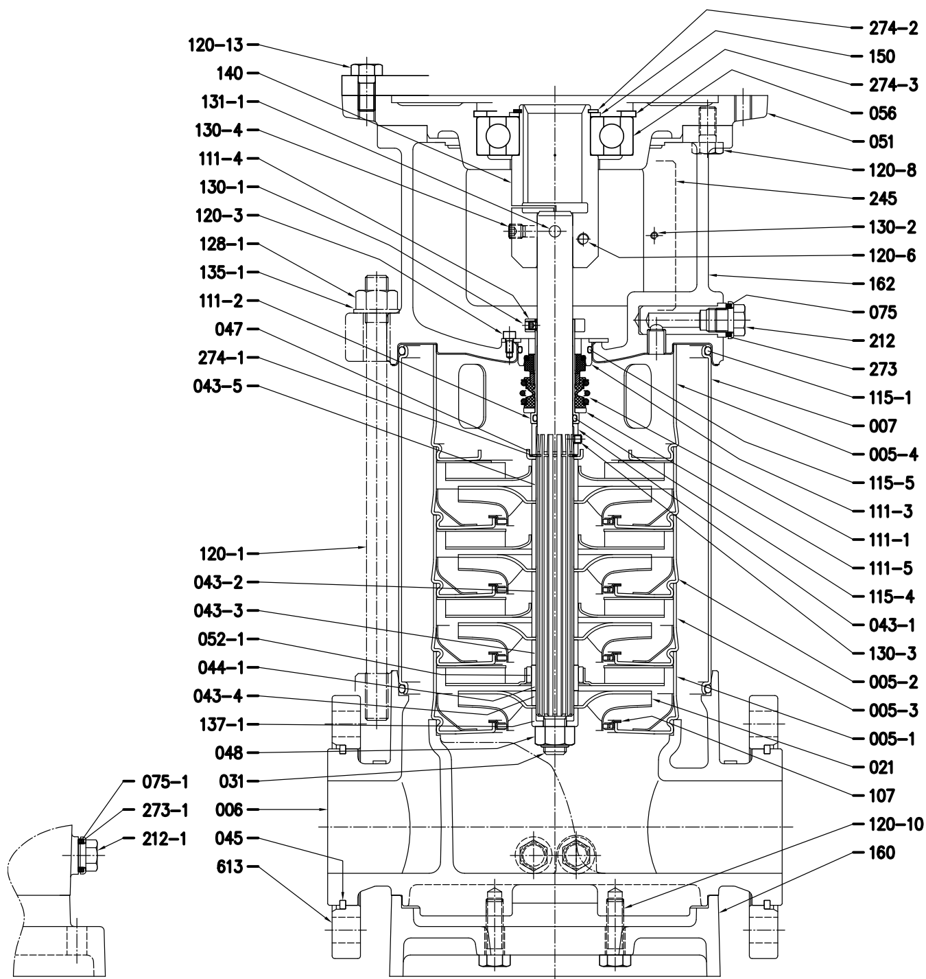
EVM(.) 32 Pump with single ball bearing
