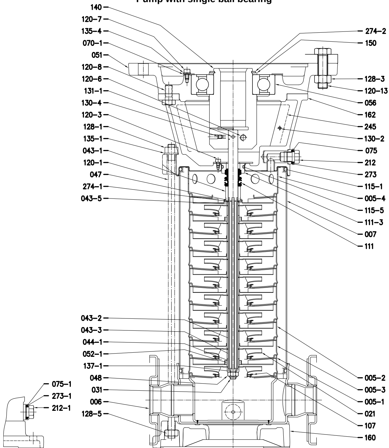
EVM(.) 10 Pump with single ball bearing
