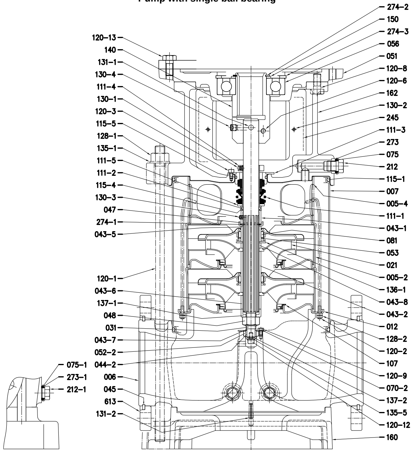
EVM(.) 64 Pump with single ball bearing
