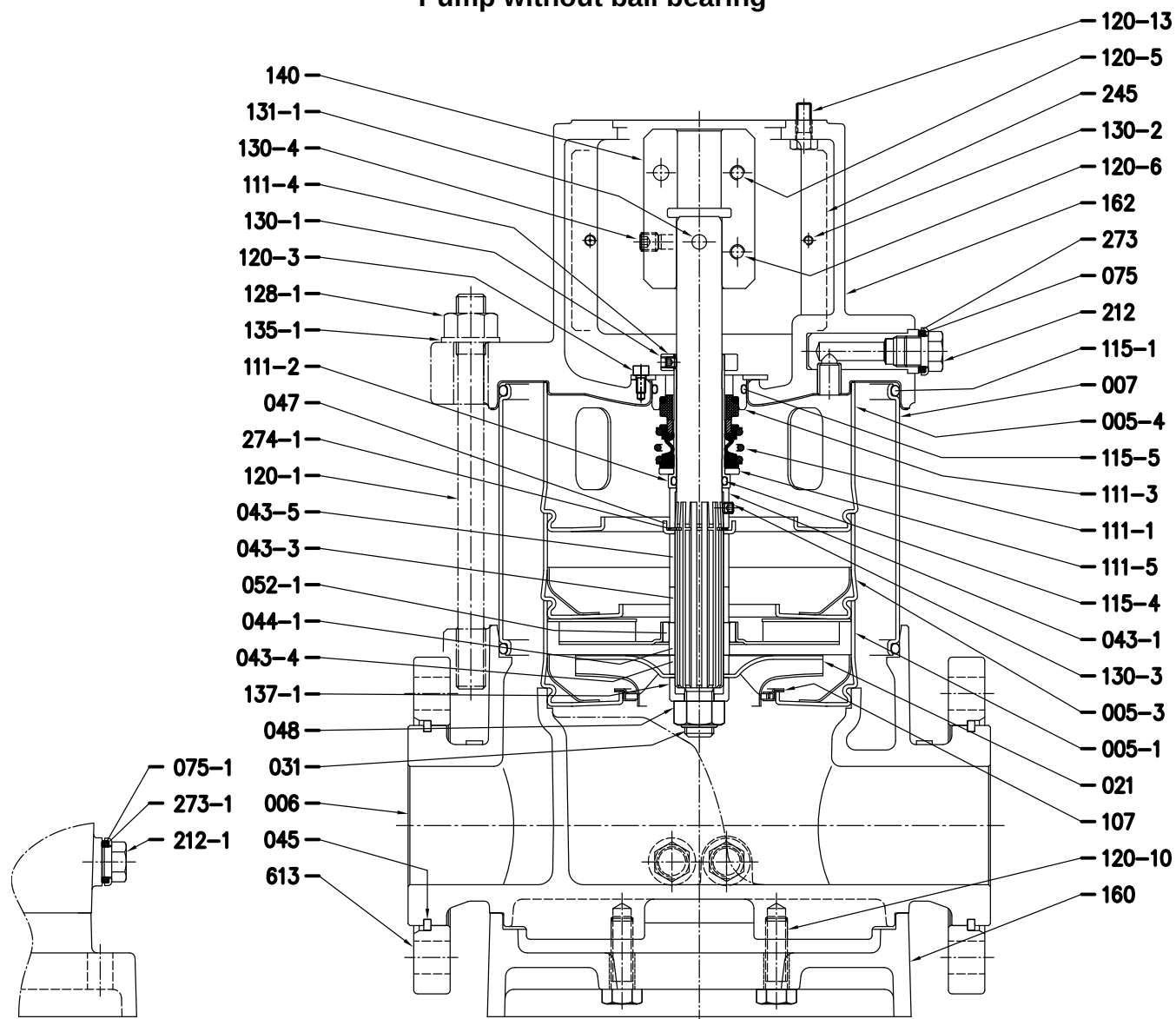
EVM(.) 32 Pump without ball bearing
